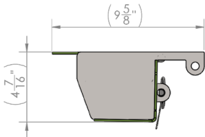
SIDE VIEW SCALE 1:4
